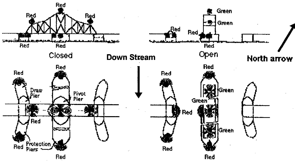
THROUGH-TYPE SWING BRIDGE (1 MARKED NAVIGATION OPENING)
