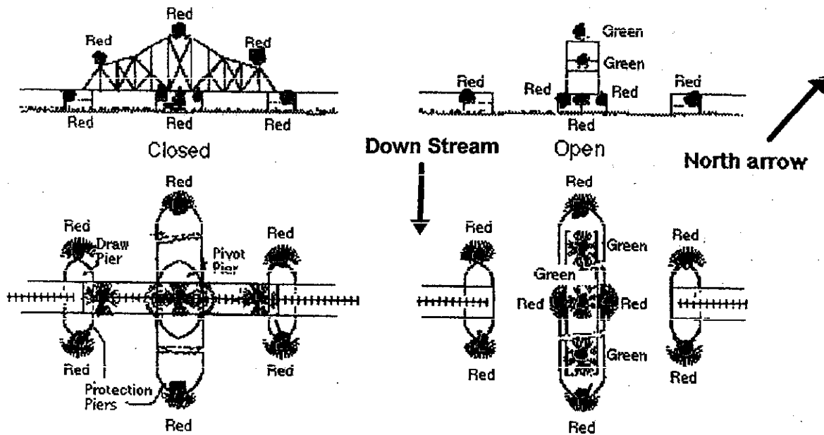
THROUGH-TYPE SWING BRIDGE (AXIS LIGHTS ONLY ON PIVOT PIER)
