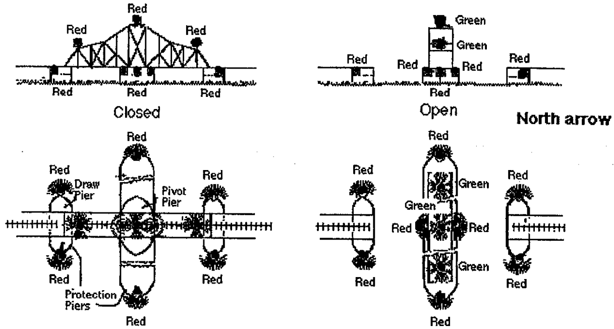
THROUGH-TYPE SWING BRIDGE (AXIS LIGHTS ONLY ON PIVOT PIER)
