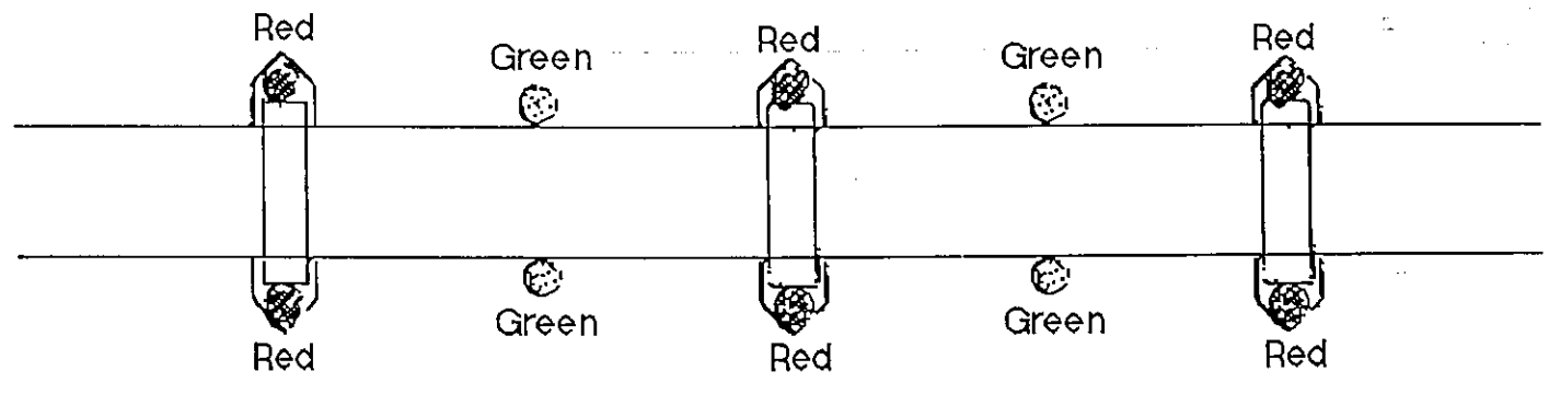
FIXED BRIDGE (2 MARKED NAVIGATION OPENINGS) (NO AXIS LIGHTS)
